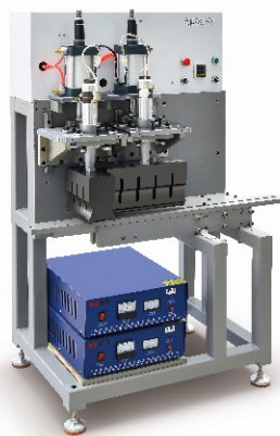
立体袋超正波封边打样机器 Ultrasonic Sealing Prototype Machine
